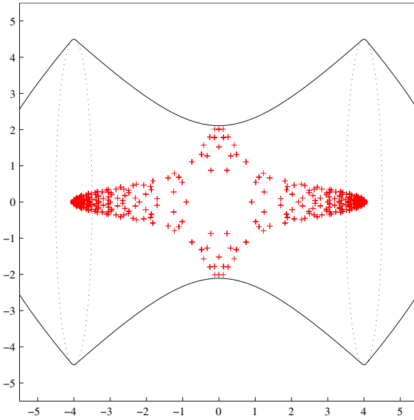
Figure 11: Spectrum of the NSA operator of Example 6.8.
