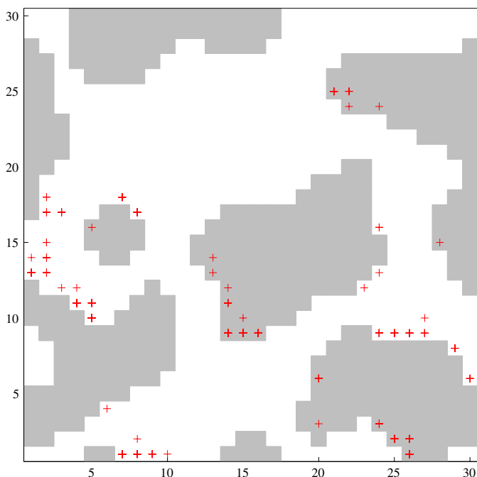
Figure 7: Distribution of the maxima of the eigenfunctions of Example 6.4.
