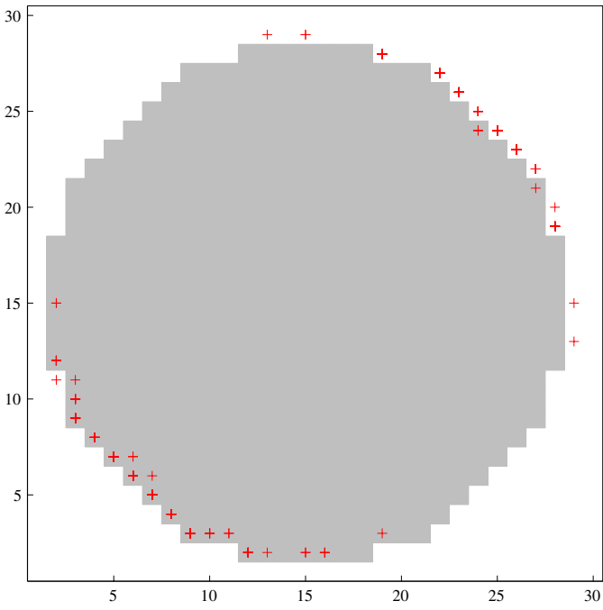
Figure 8: Distribution of the maxima of the eigenfunctions of Example 6.1.
