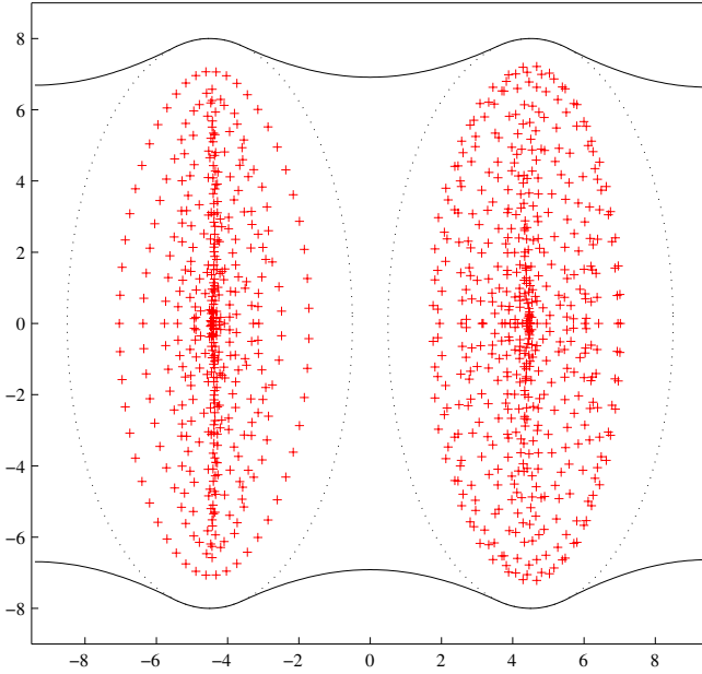
Figure 5: Spectrum of the NSA operator of Example 6.3.
