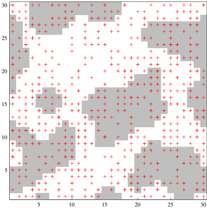
Figure 9: Distribution of the maxima of the eigenfunctions of Example 6.6.
