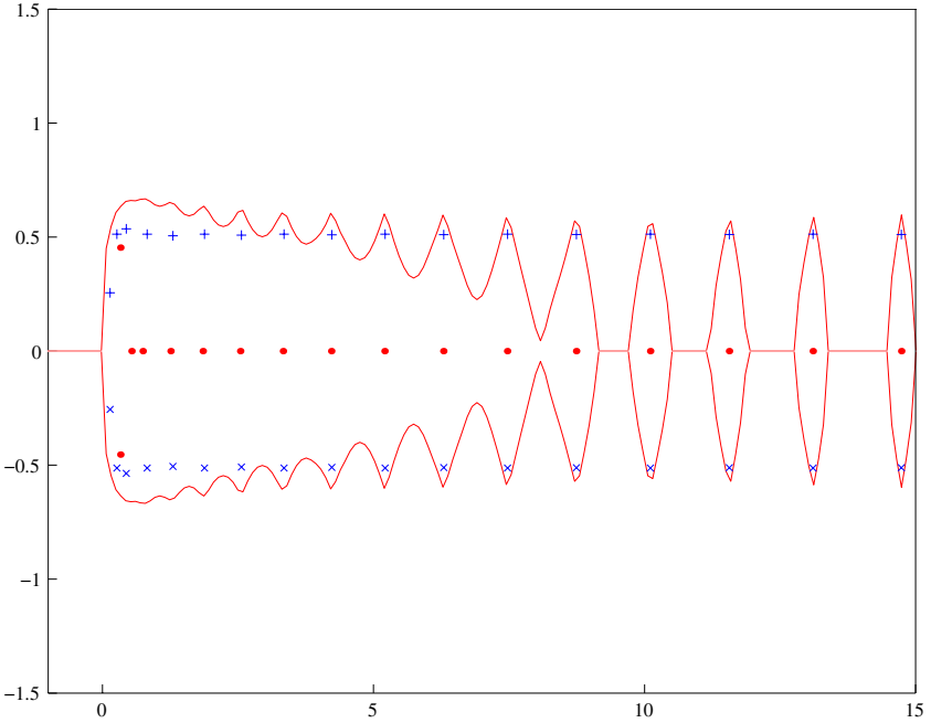
Figure 1: The set T for -1 < x < 15 .
