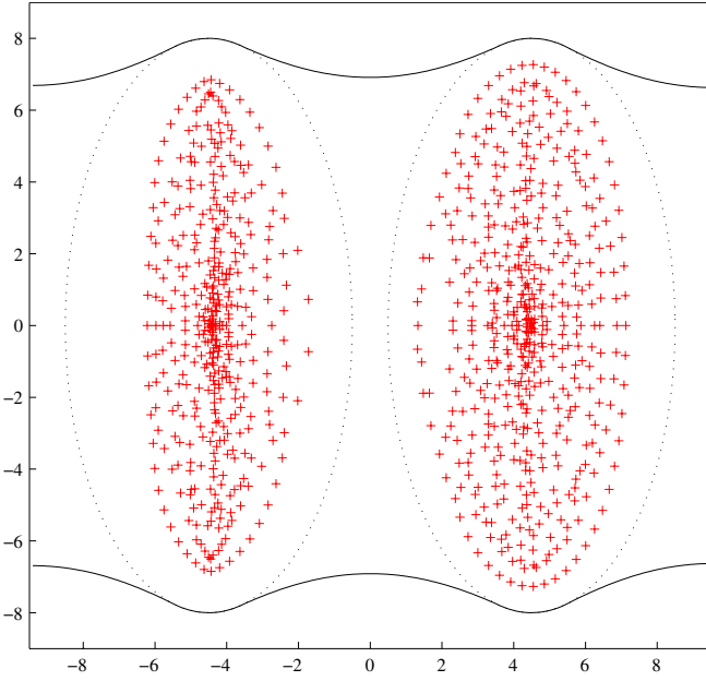
Figure 6: Spectrum of the NSA operator of Example 6.4.
