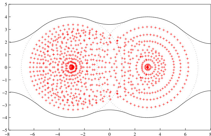
Figure 3: Spectrum of the NSA operator of Example 6.1.
