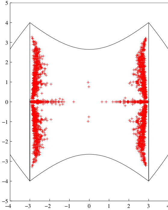
Figure 10: Spectrum of the NSA operator of Example 6.7.
