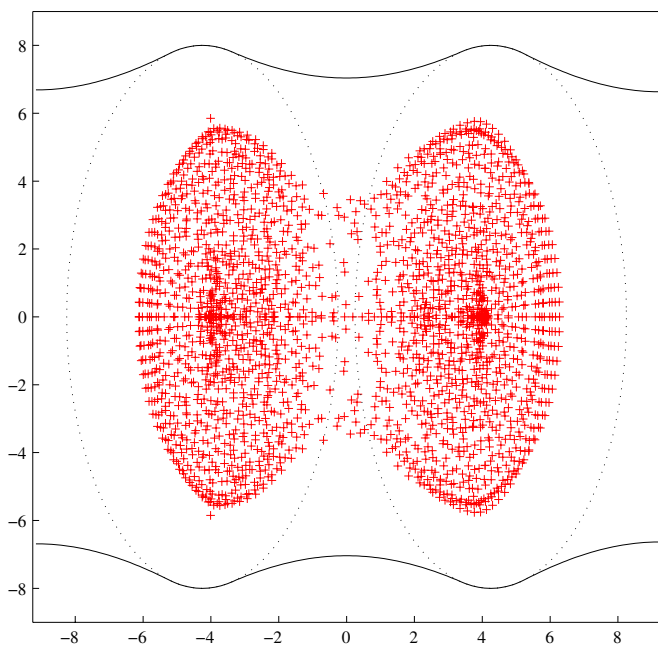
Figure 4: Spectrum of the NSA operator of Example 6.2.
